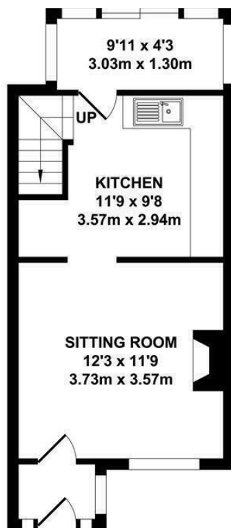
GROUND FLOOR APPROX. FLOOR AREA 328 SQ.FT. (30.44 SQ.M.)
